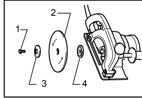
1. Hex bolt 2. Diamond wheel 3. Outer flange 4. Inner flange
