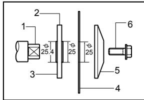
1. Mounting shaft 2. Inner flange 3. 25.4 mm marking 4. Diamond wheel 5. Outer flange 6. Hex bolt
