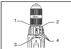
1. Adjusting ring 2. Drill marking 3. Pointer 4. Graduations
