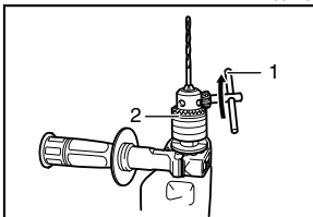
1. Chuck key 2. Chuck
