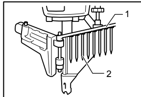
1. Slot 2. Feeder body
