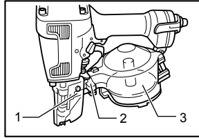
1. Door 2. Latch lever 3. Magazine cap
