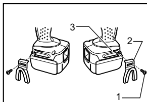
1. Vis 2. Crochet 3. Rainure
