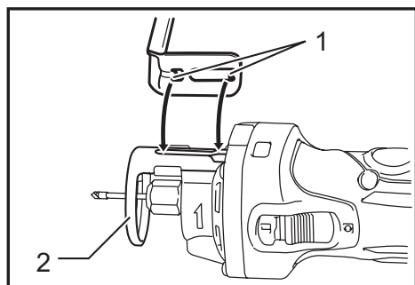
► 1. Projections 2. Shoe
