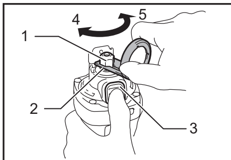
► 1. Collet nut 2. Shoe 3. Shaft lock 4. Tighten 5. Loosen
