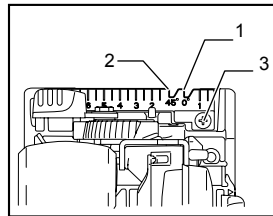
1. Cutting line (0° position) 2. Cutting line (45° position) 3. Screw
