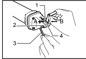
1. Center blade 2. Bolt 3. Hex wrench 4. Side blade
