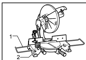
1. Holder 2. Screw
