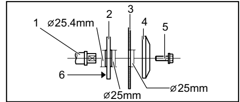
1. Spindle 2. Inner flange 3. Blade 4. Outer flange 5. Hex bolt 6. 25.4 mm marking
