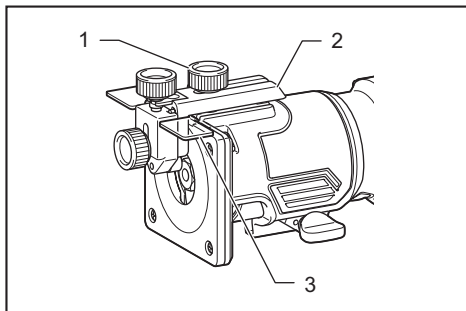
► 1. Clamping screw 2. Guide holder 3. Chip deflector
