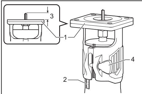
► 1. Base 2. Scale 3. Bit protrusion 4. Clamping screw
