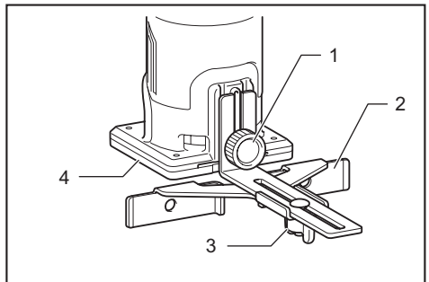
► 1. Clamping screw 2. Straight guide 3. Wing nut 4. Base
