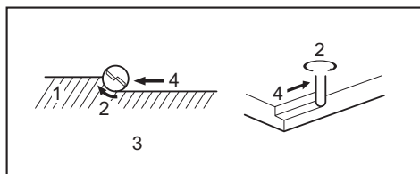
► 1. Workpiece 2. Bit revolving direction 3. View from the top of the tool 4. Feed direction
